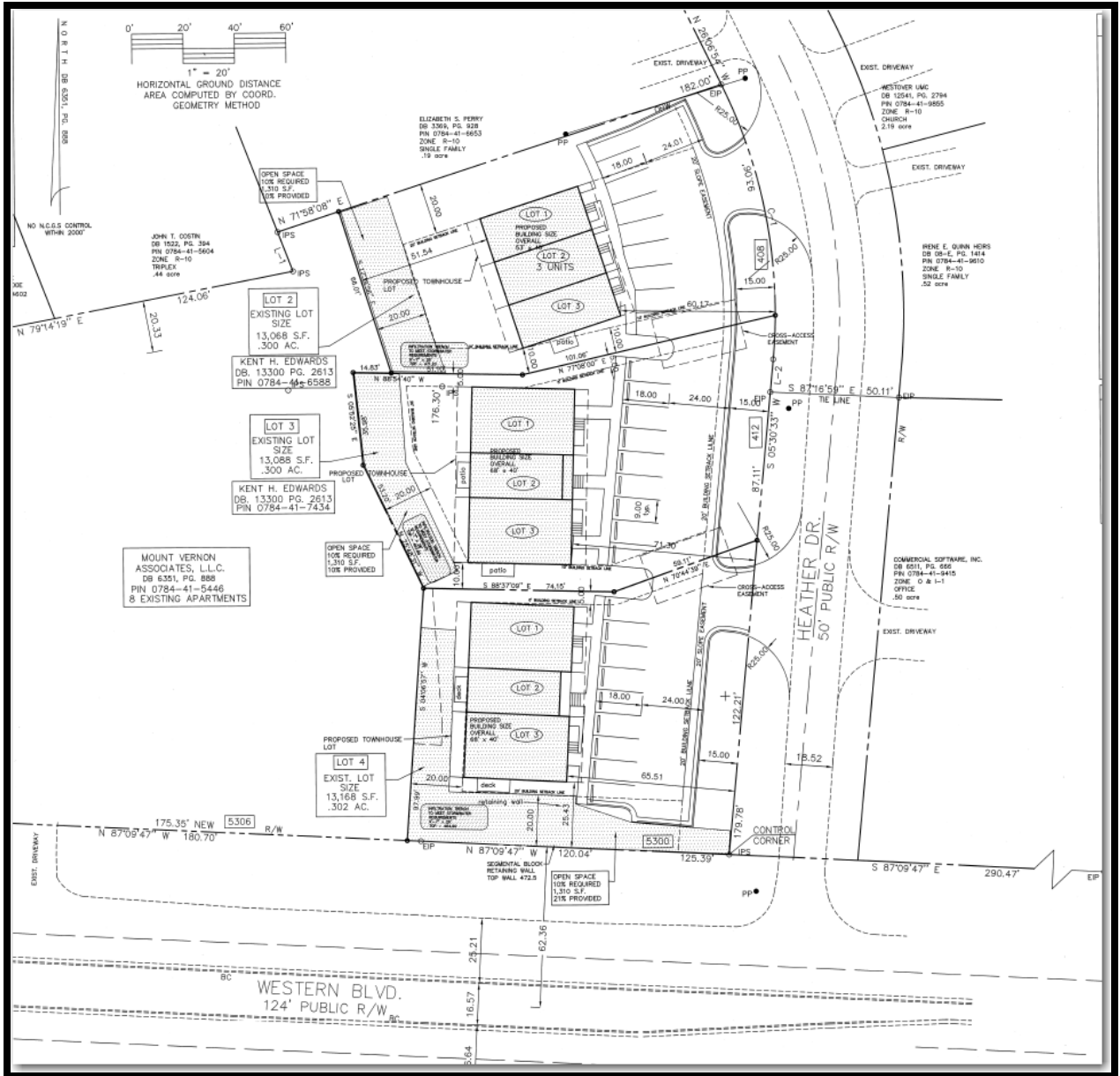
S-39-10 Edwards Townhomes lot 4 - subdivision plan
