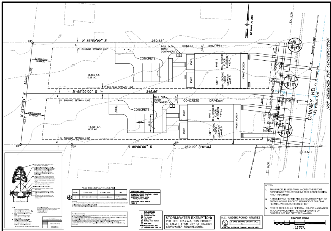
SR-57-16 Preliminary Site Plan
