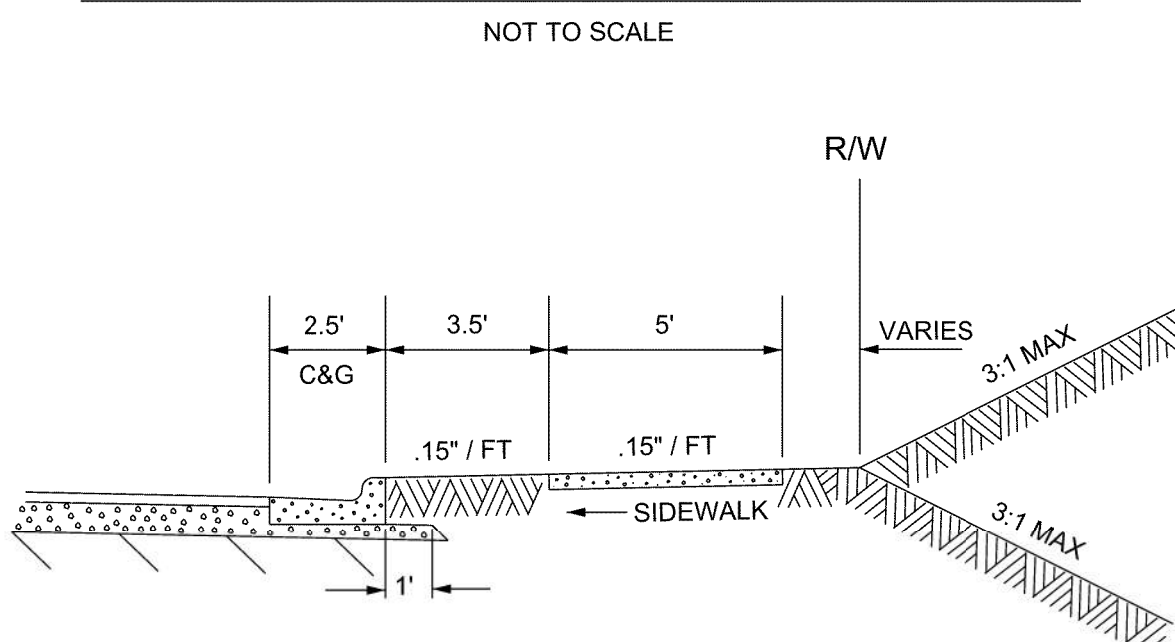
TYPICAL SIDEWALK SECTION
