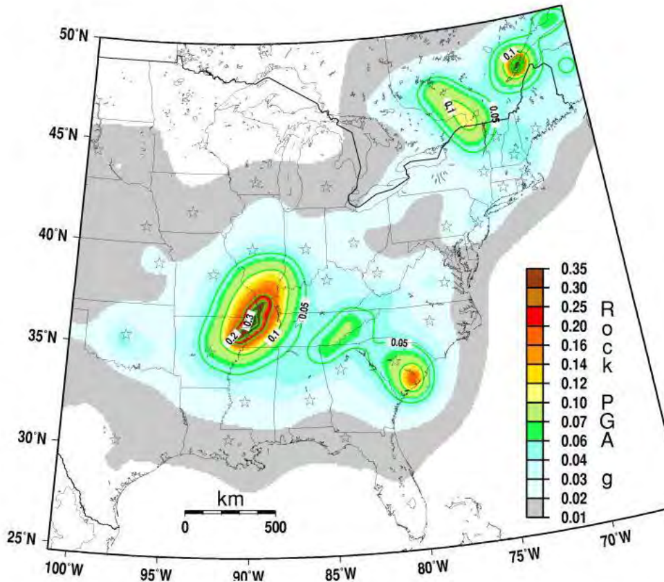
FIGURE K.3: PEAK ACCELERATION WITH 10 PERCENT PROBABILITY OF EXCEEDANCE IN 50 YEARS
