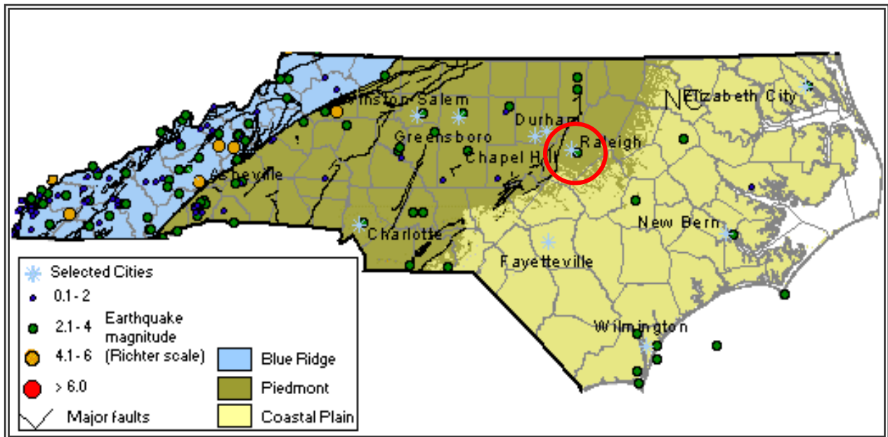
FIGURE I.2: GEOLOGICAL AND SEISMIC INFORMATION FOR NORTH CAROLINA
