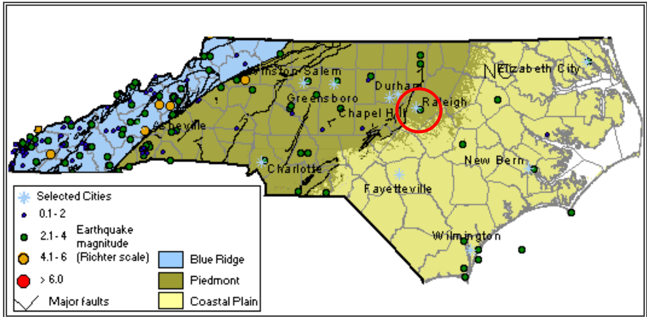
FIGURE K.2: GEOLOGICAL AND SEISMIC INFORMATION FOR NORTH CAROLINA
