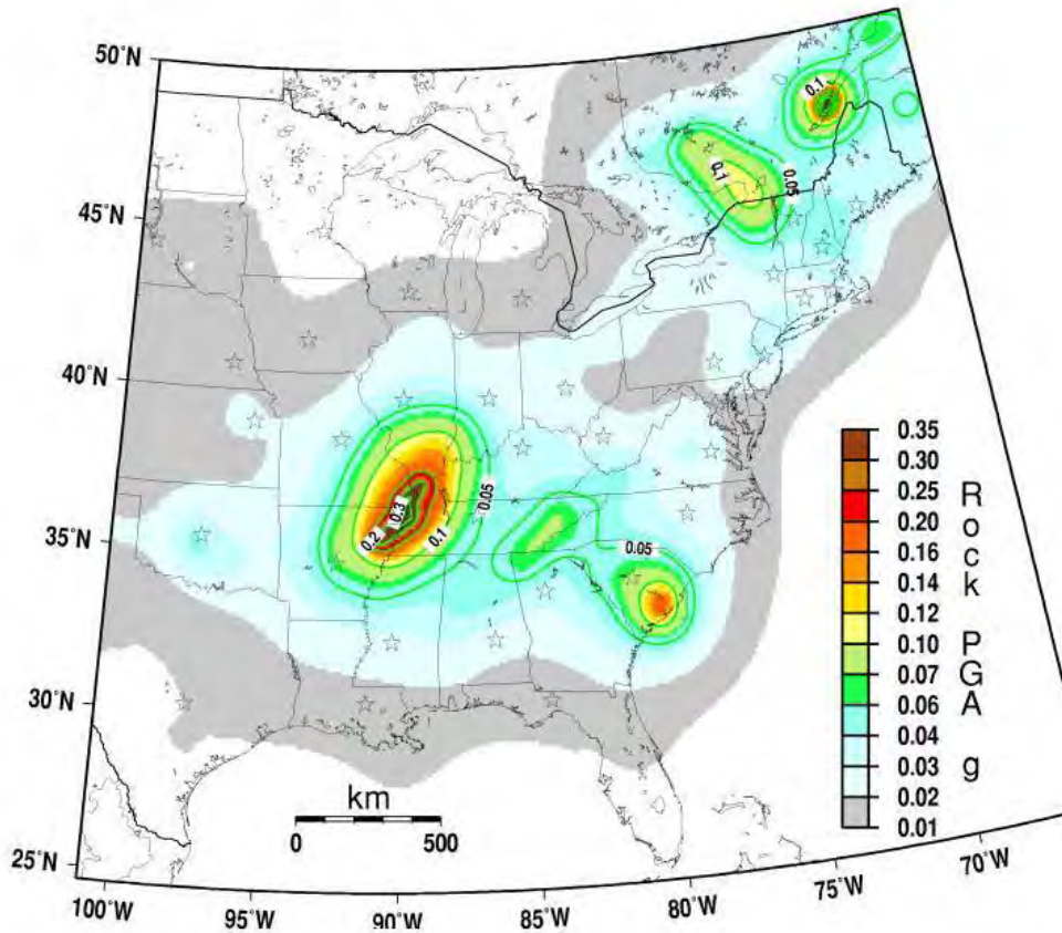
FIGURE H.3: PEAK ACCELERATION WITH 10 PERCENT PROBABILITY OF EXCEEDANCE IN 50 YEARS
