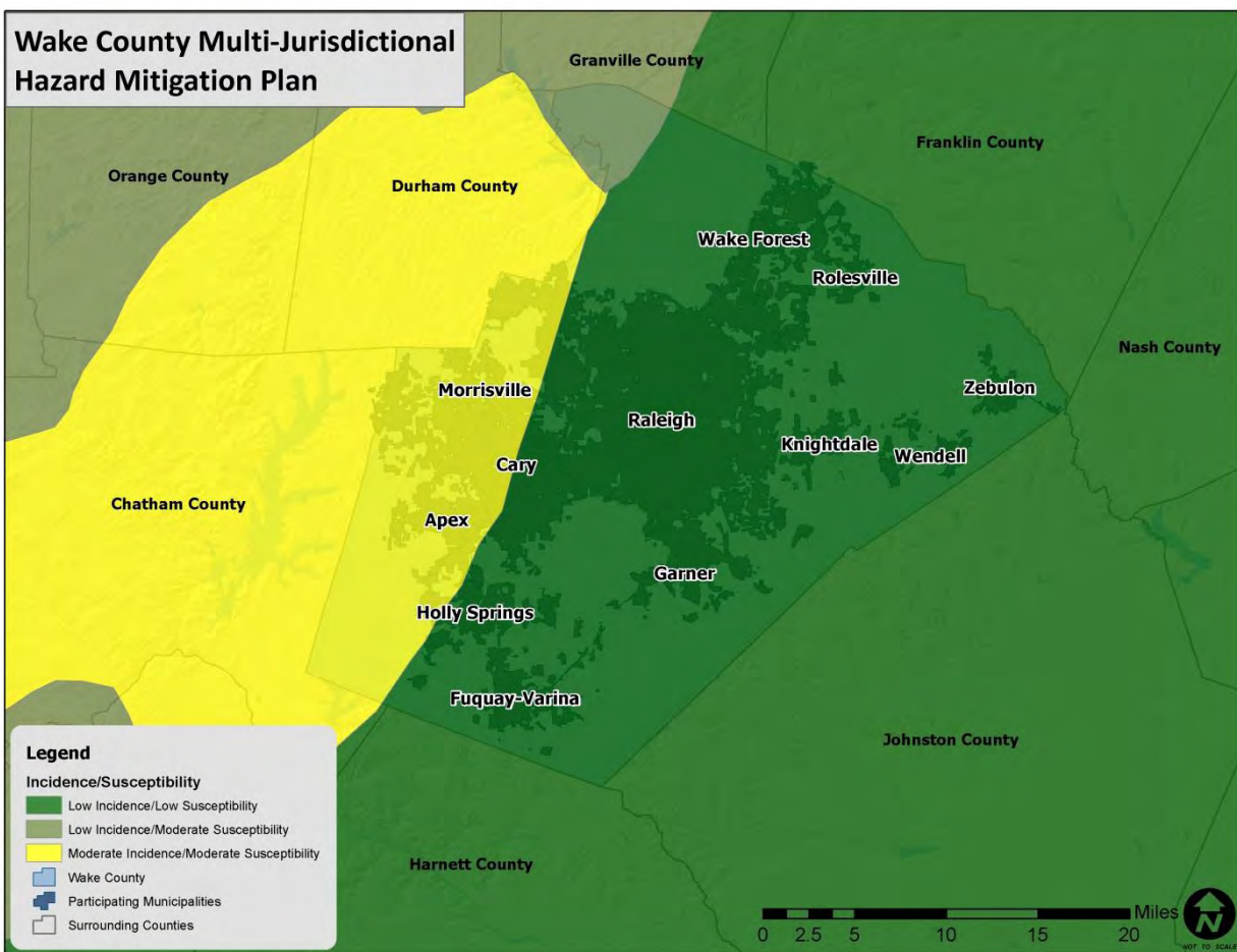
FIGURE E.4: LANDSLIDE SUSCEPTIBILITY AND INCIDENCE MAP OF WAKE COUNTY
