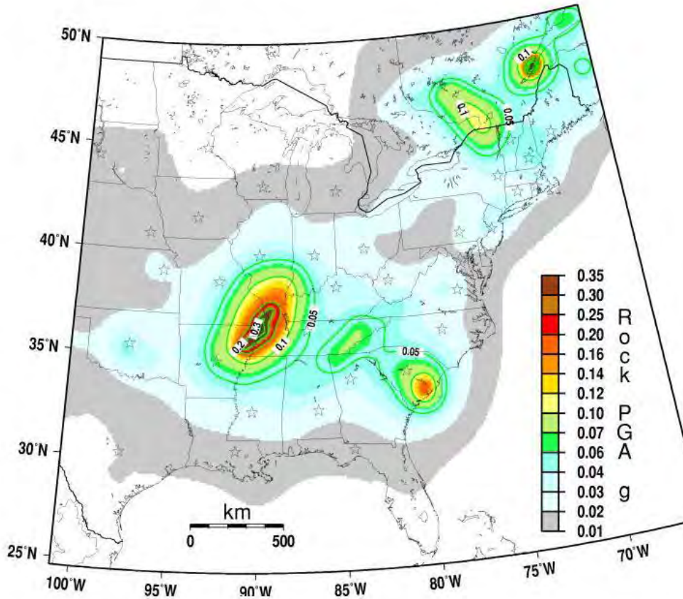
FIGURE I.3: PEAK ACCELERATION WITH 10 PERCENT PROBABILITY OF EXCEEDANCE IN 50 YEARS
