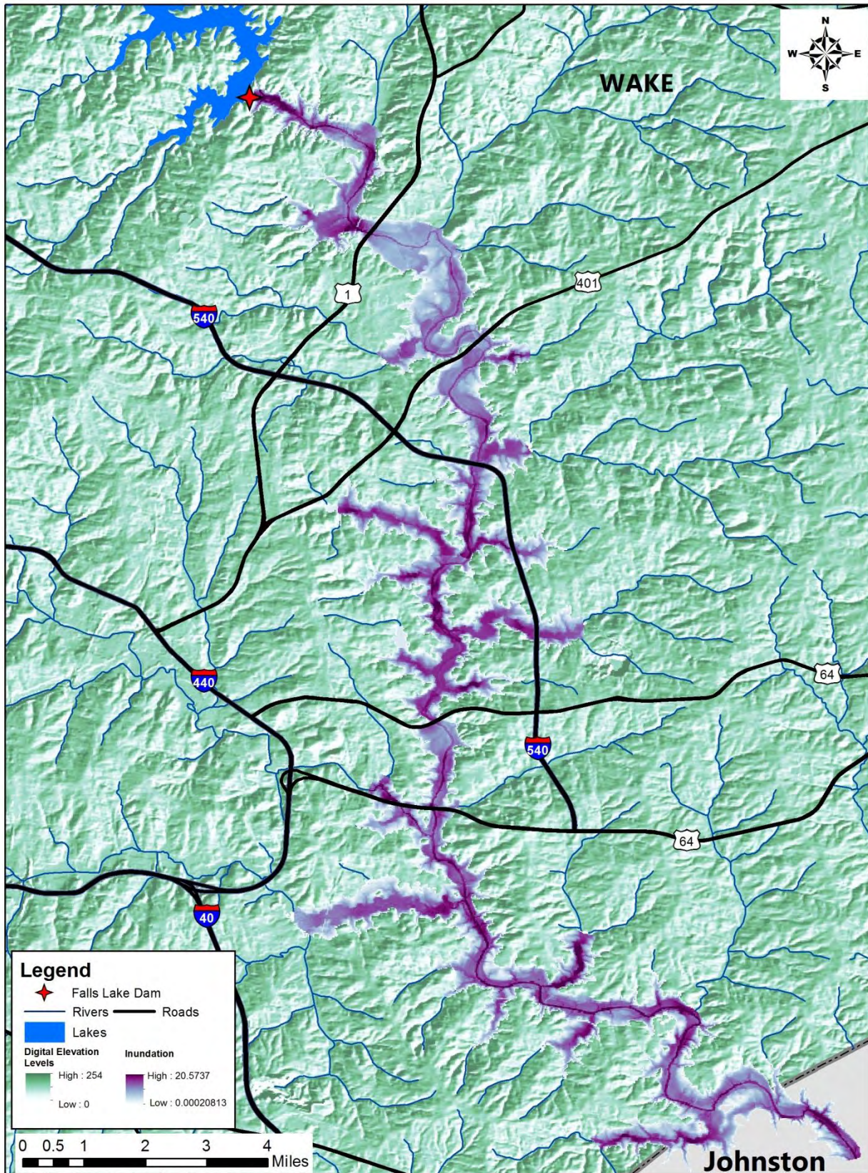
FIGURE 5.15: FALLS LAKE DAM FAILURE INUNDATION AREA
