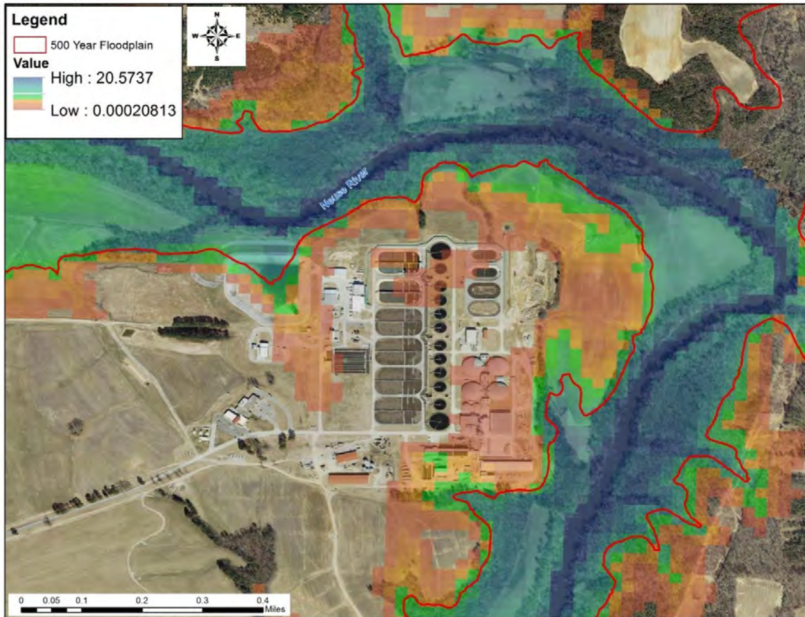
FIGURE 5.16: INUNDATION OF THE NEUSE RIVER WASTEWATER TREATMENT PLANT
