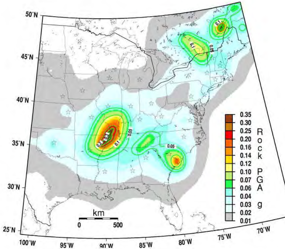
FIGURE L.3: PEAK ACCELERATION WITH 10 PERCENT PROBABILITY OF EXCEEDANCE IN 50 YEARS
