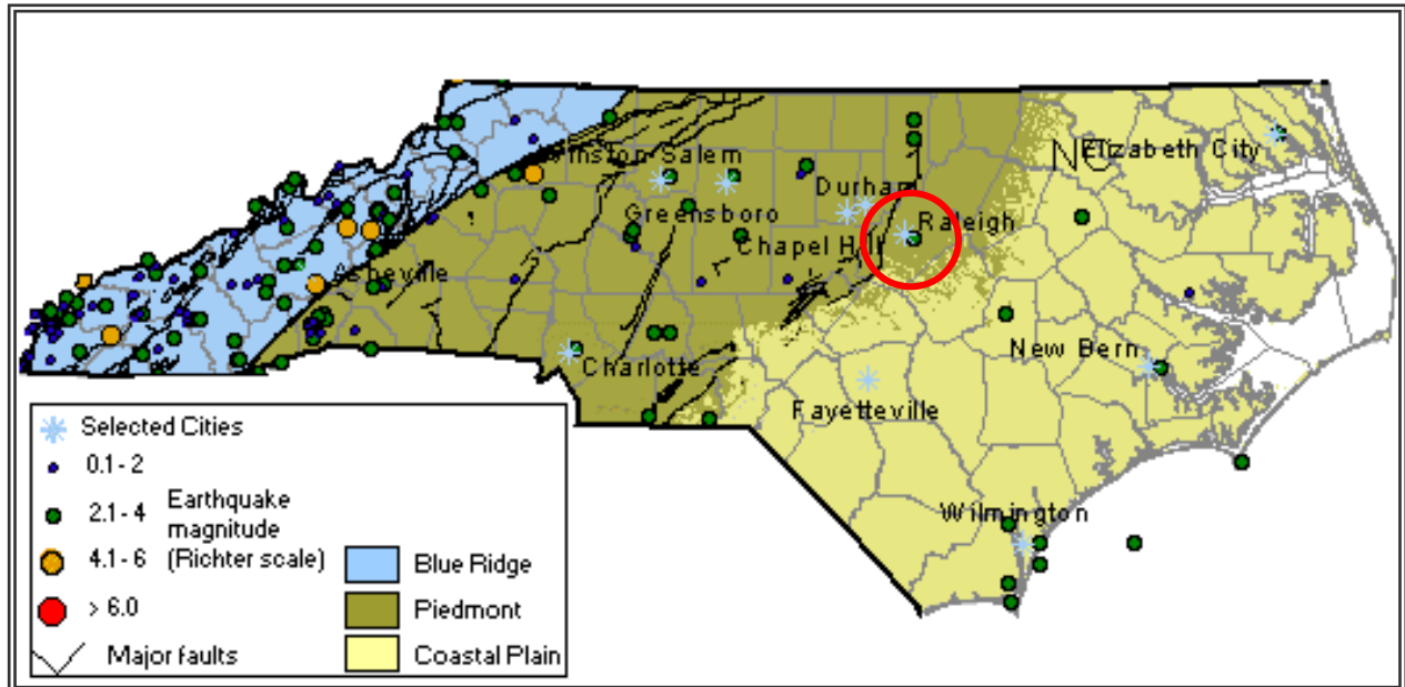
FIGURE M.2: GEOLOGICAL AND SEISMIC INFORMATION FOR NORTH CAROLINA
