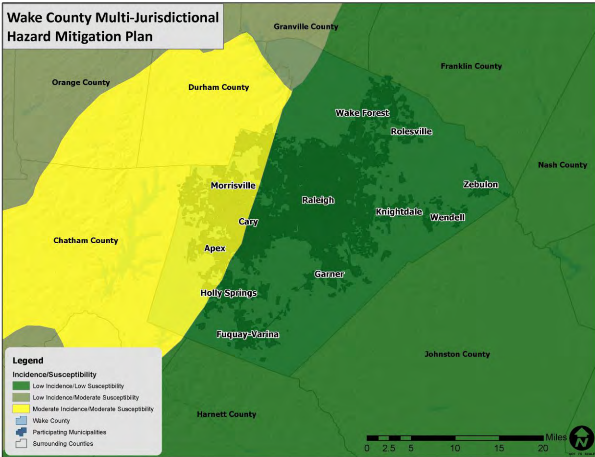
FIGURE 5.11: LANDSLIDE SUSCEPTIBILITY AND INCIDENCE MAP OF WAKE COUNTY
