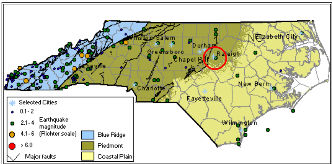
FIGURE L.2: GEOLOGICAL AND SEISMIC INFORMATION FOR NORTH CAROLINA
