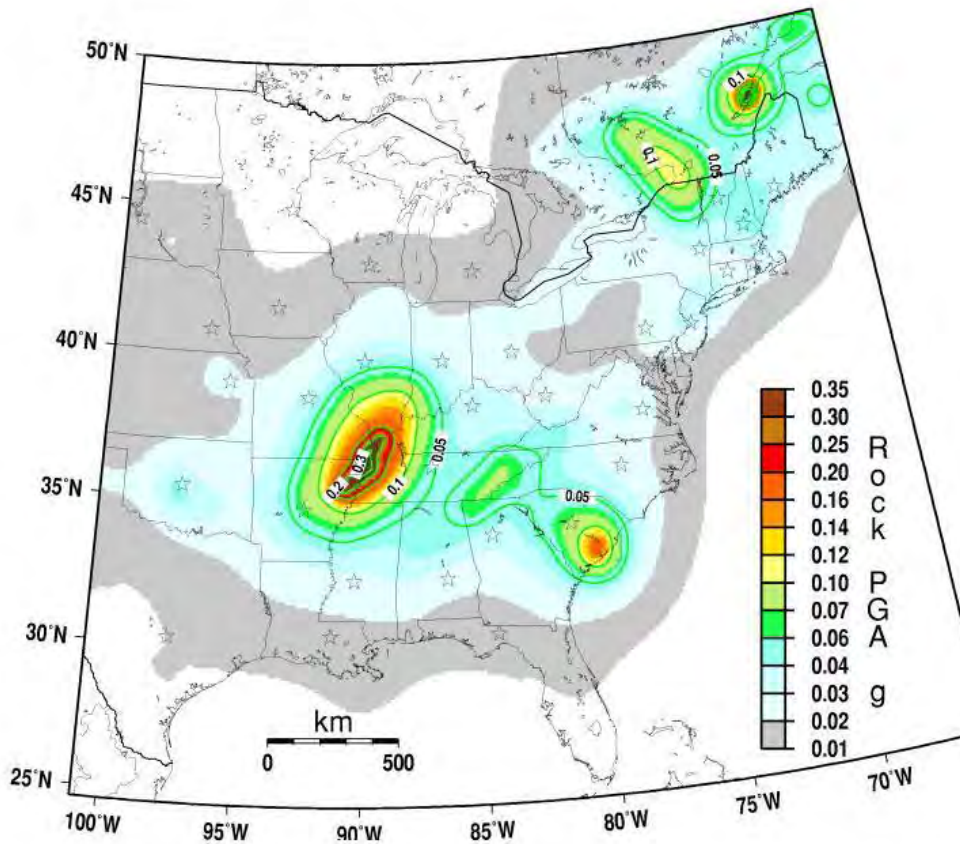
FIGURE G.3: PEAK ACCELERATION WITH 10 PERCENT PROBABILITY OF EXCEEDANCE IN 50 YEARS
