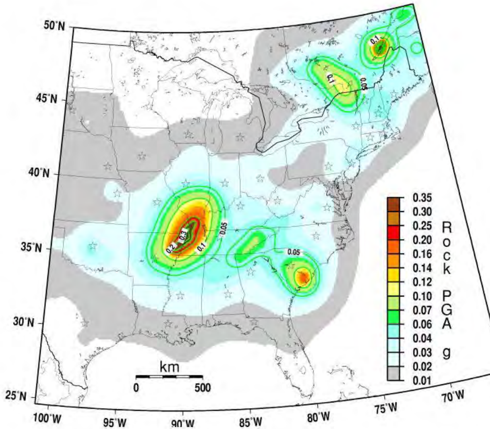
FIGURE M.3: PEAK ACCELERATION WITH 10 PERCENT PROBABILITY OF EXCEEDANCE IN 50 YEARS
