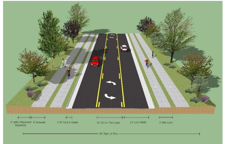
Typical Section Alternative 2
