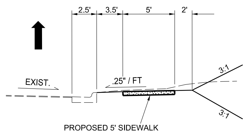
TYPICAL SIDEWALK SECTION (NOT TO SCALE)
