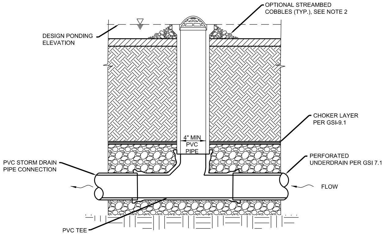
BIORETENTION SECTION WITH OVERFLOW
