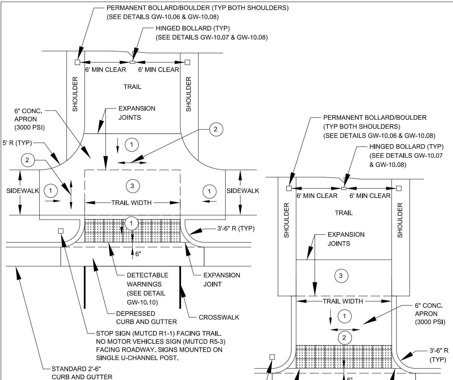
TRAIL TIE-IN WITH SIDEWALK
