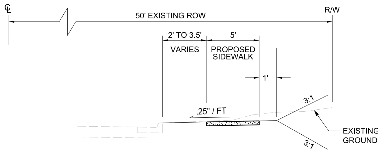
TYPICAL SIDEWALK SECTION - RIGHT (NOT TO SCALE)
