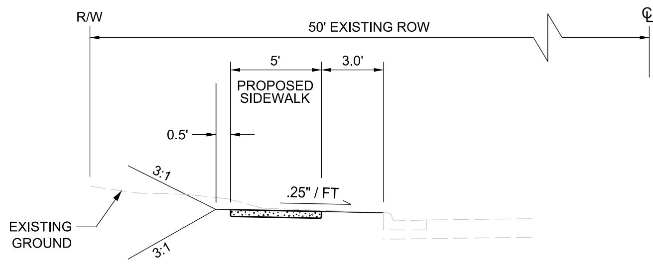
TYPICAL SIDEWALK SECTION - LEFT (NOT TO SCALE)
