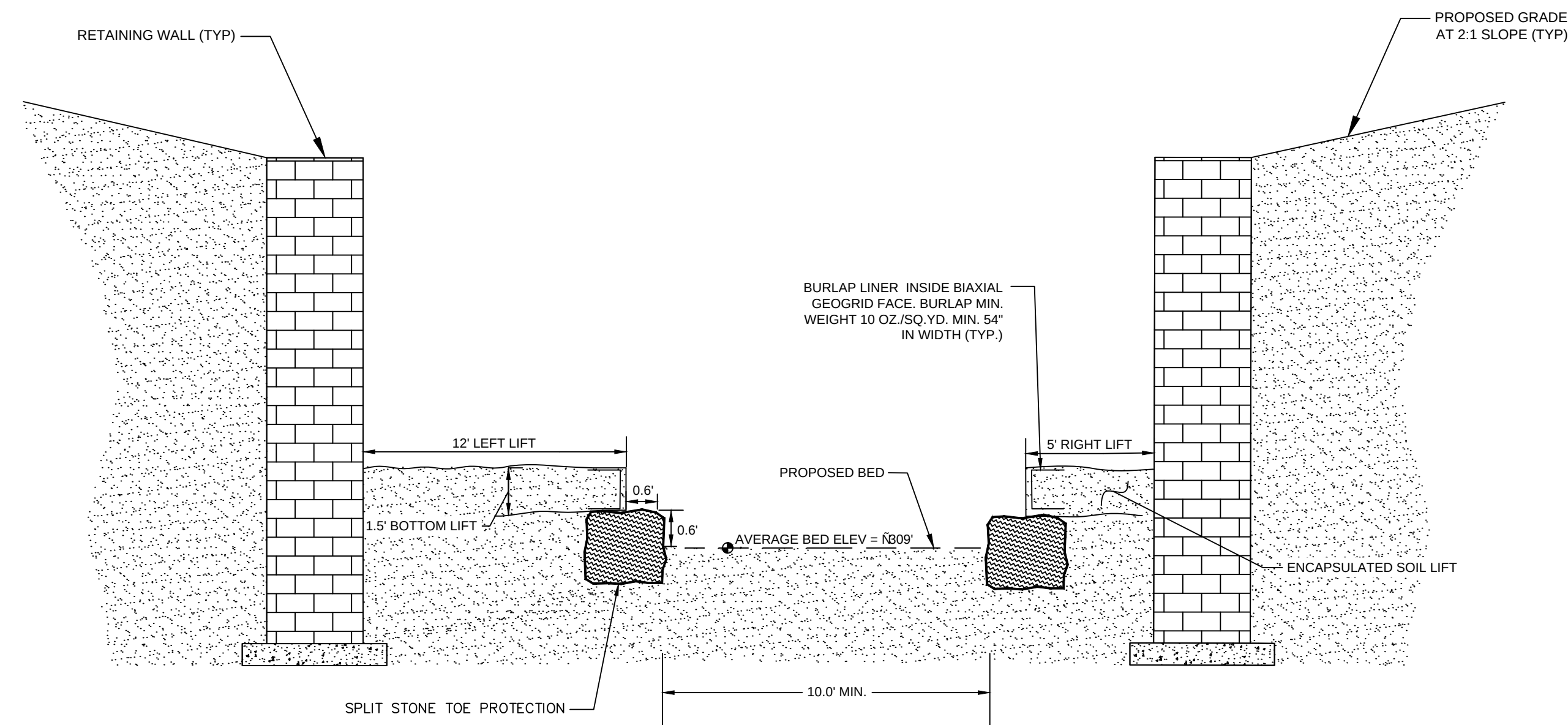
RETAINING WALL DETAIL LOOKING DOWNSTREAM (NOT TO SCALE)
