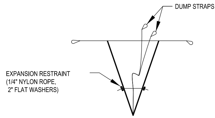
BAG DETAIL
