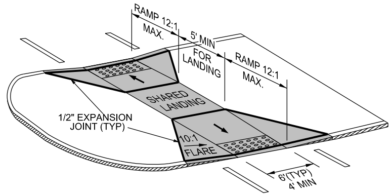
MEDIAN ISLAND CURB RAMPS (MEDIANS WIDER THAN 20')
