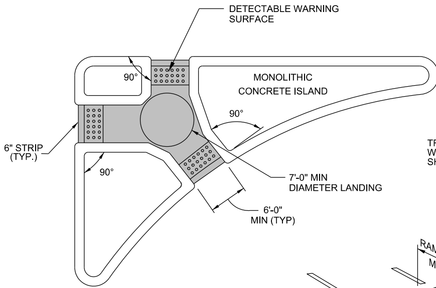
TRIANGULAR ISLAND WITH CUT THROUGH
