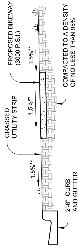
TYPICAL SECTION
