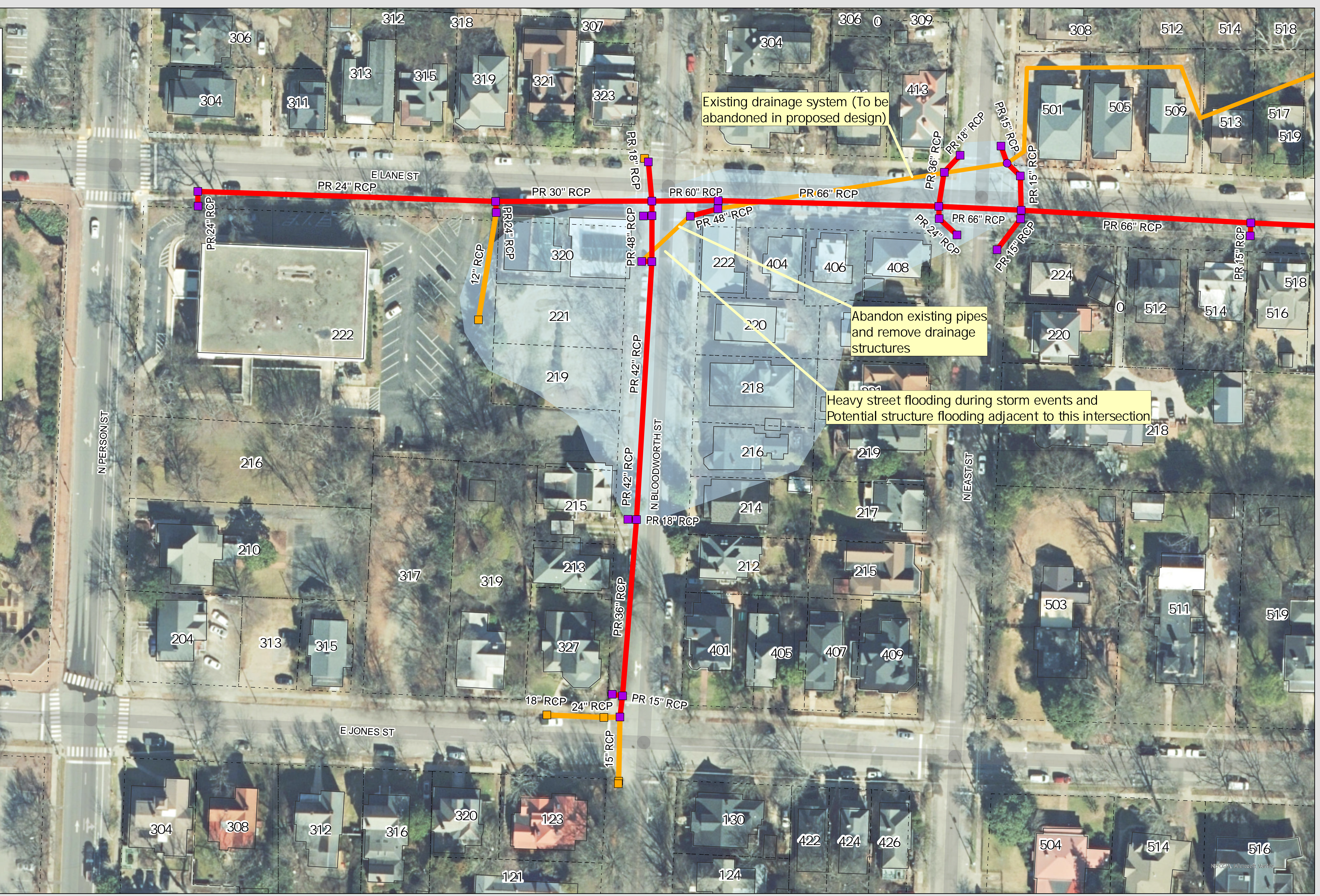
East Lane Street Drainage Improvement Project Figure 1.B - Existing vs Proposed Design (10-yr Design Storm)
