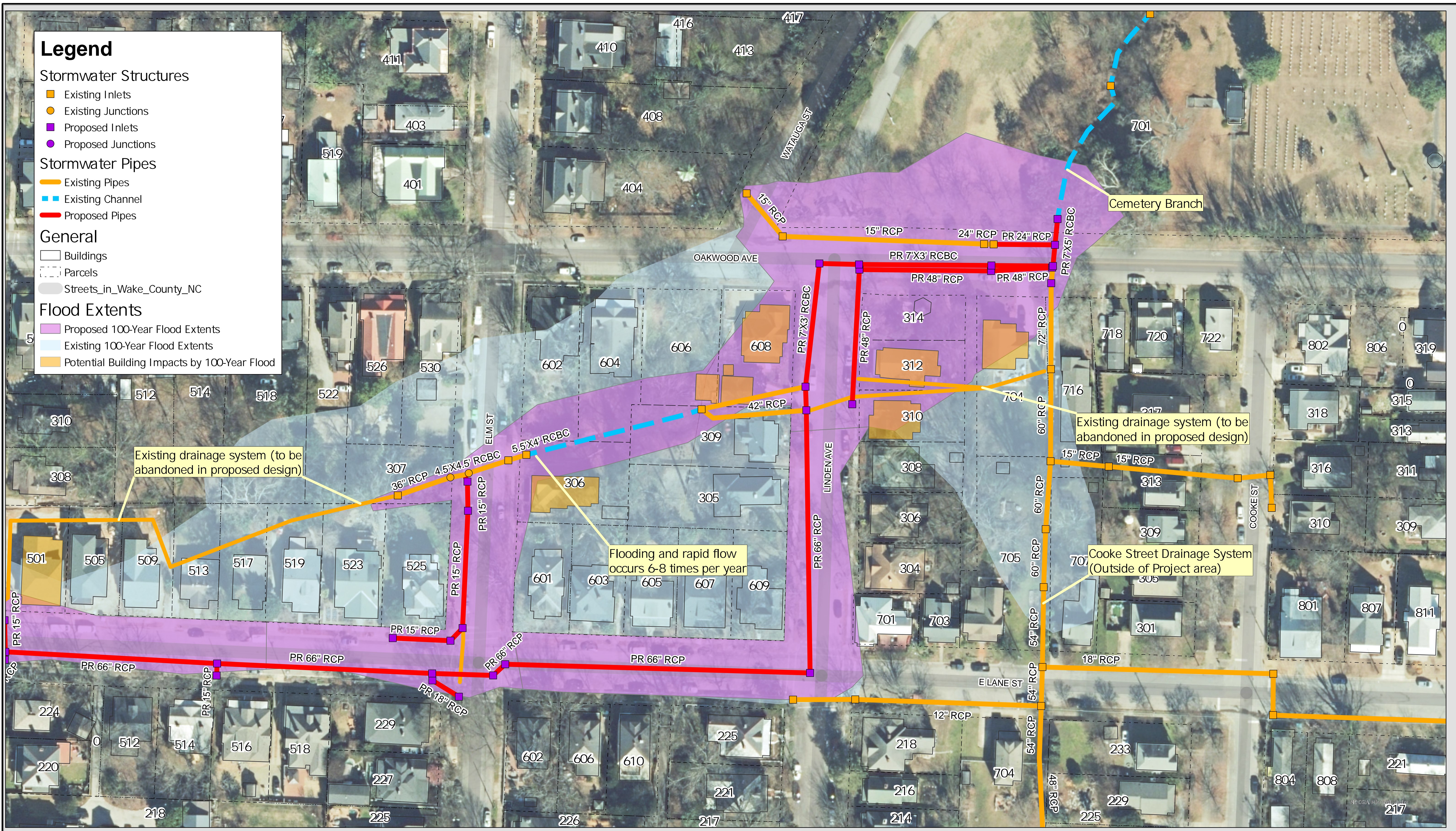
East Lane Street Drainage Improvement Project Figure 2.A - Existing vs Proposed Design (100-yr Design Storm)
