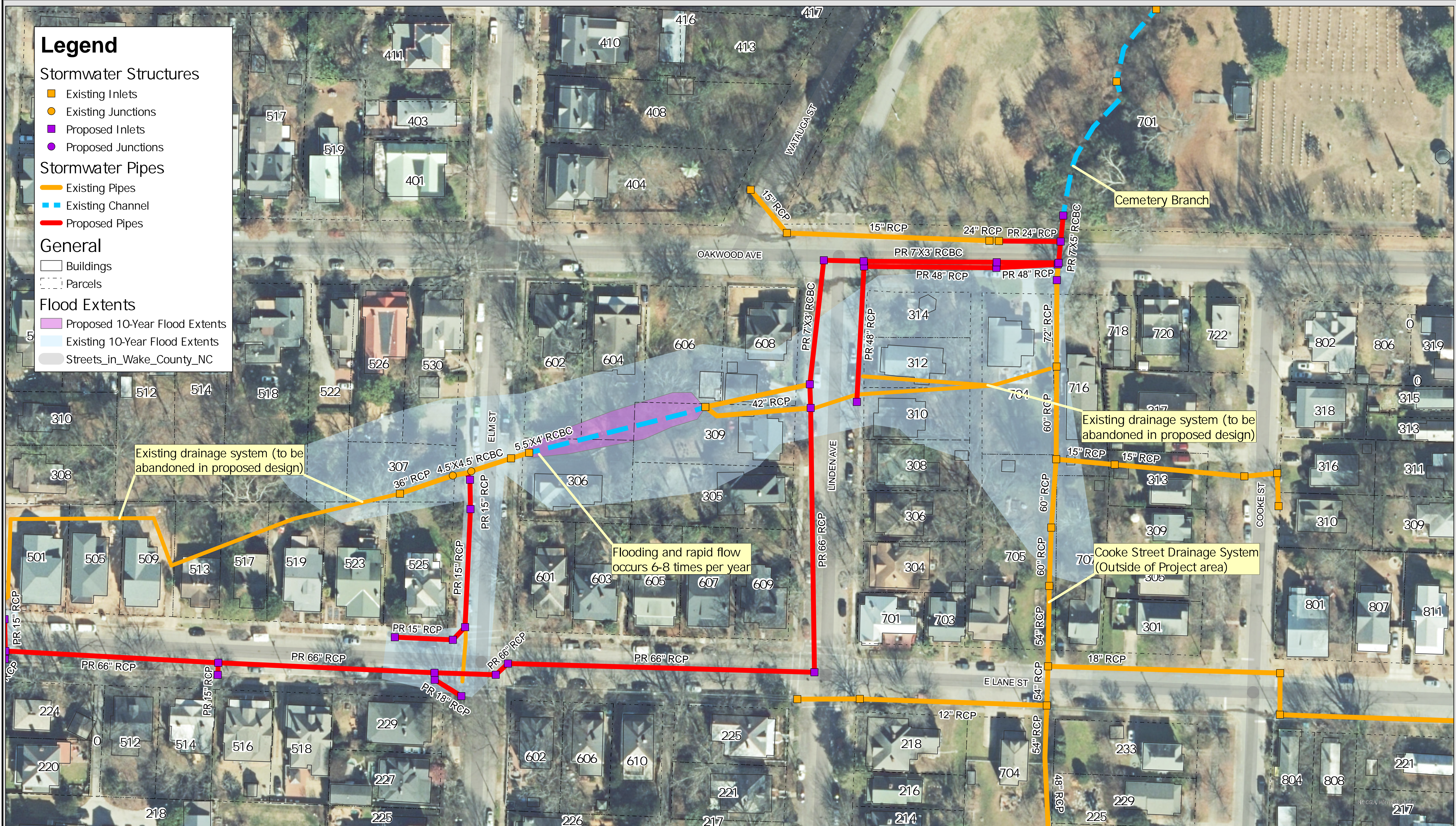
East Lane Street Drainage Improvement Project Figure 1.A - Existing vs Proposed Design (10-yr Design Storm)
