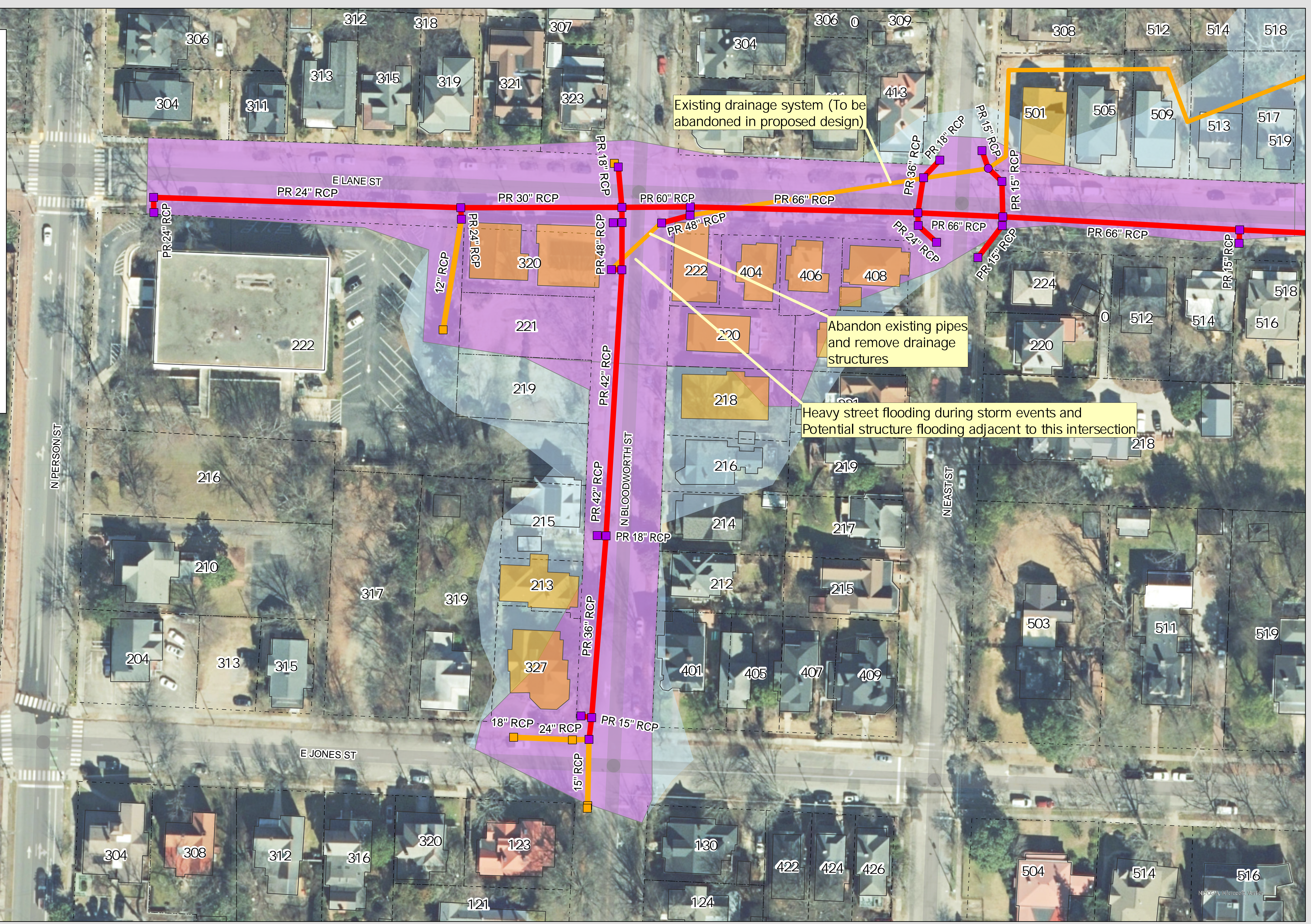
East Lane Street Drainage Improvement Project Figure 2.B - Existing vs Proposed Design (100-yr Design Storm)
