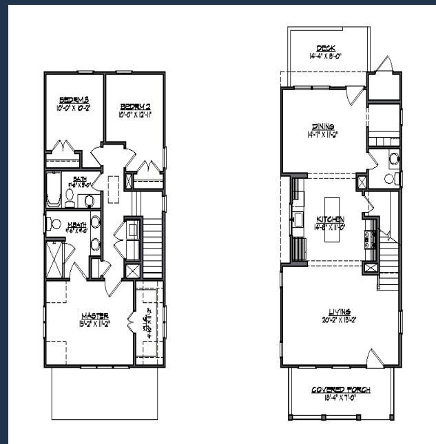
Floorplan- 2 story**
