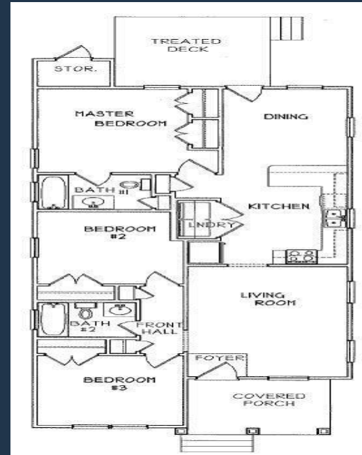
Floorplan- 1 Story**
