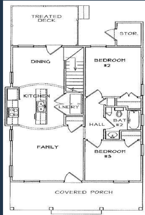
Floorplan- 2 Story**
