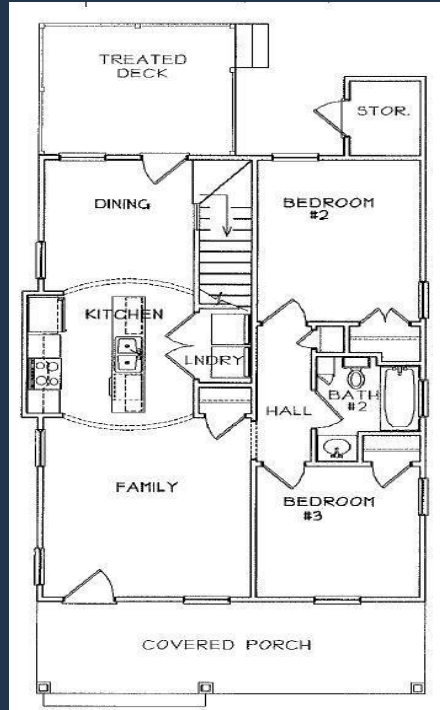
Floorplan- 2 Story**
