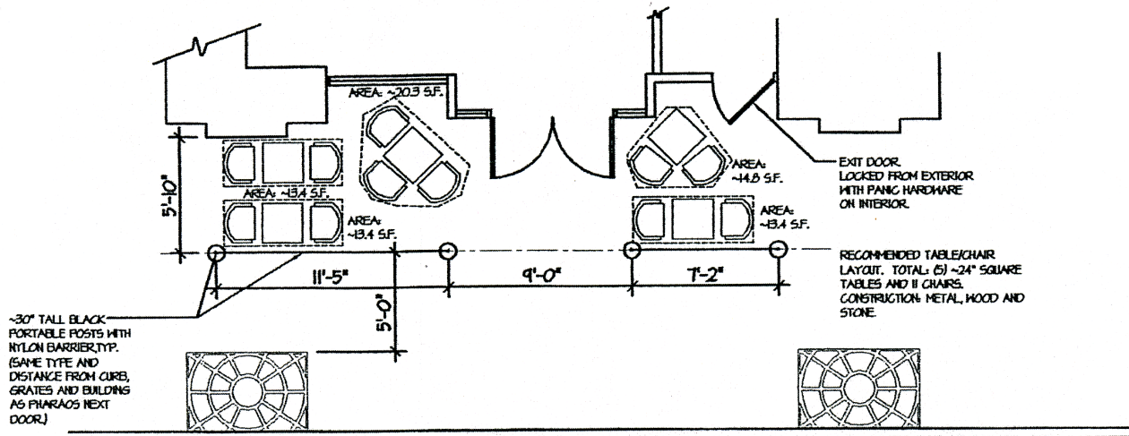
Furniture Layout 1/8" = 1'-0"
