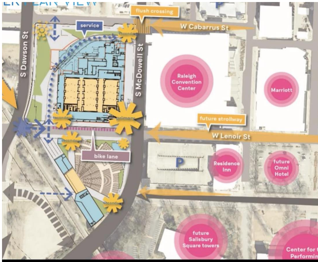
Site uses, entrances, and pedestrian paths
