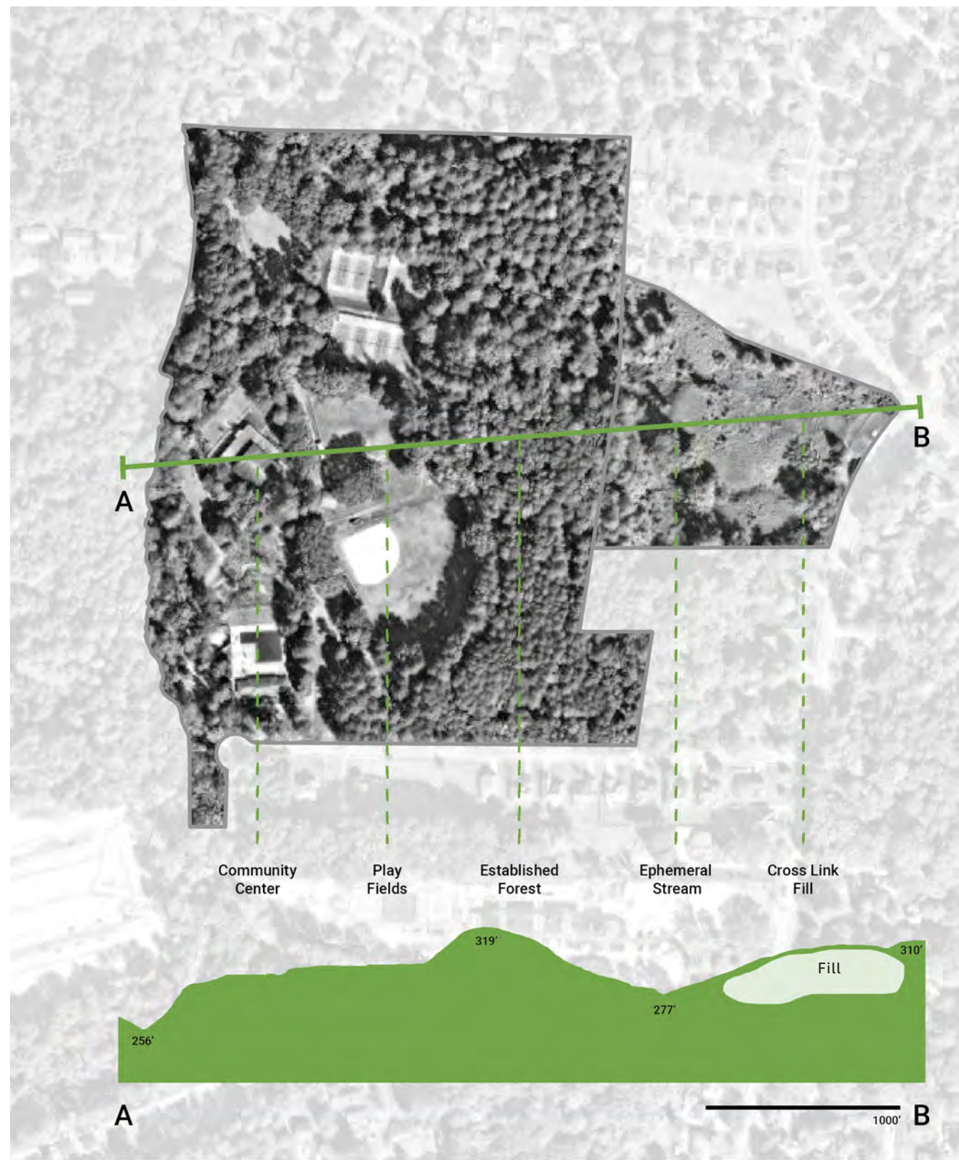
Site Topographic Section (West to East) showing Existing Park Infrastructure, Ephemeral Stream, and Fill Material
