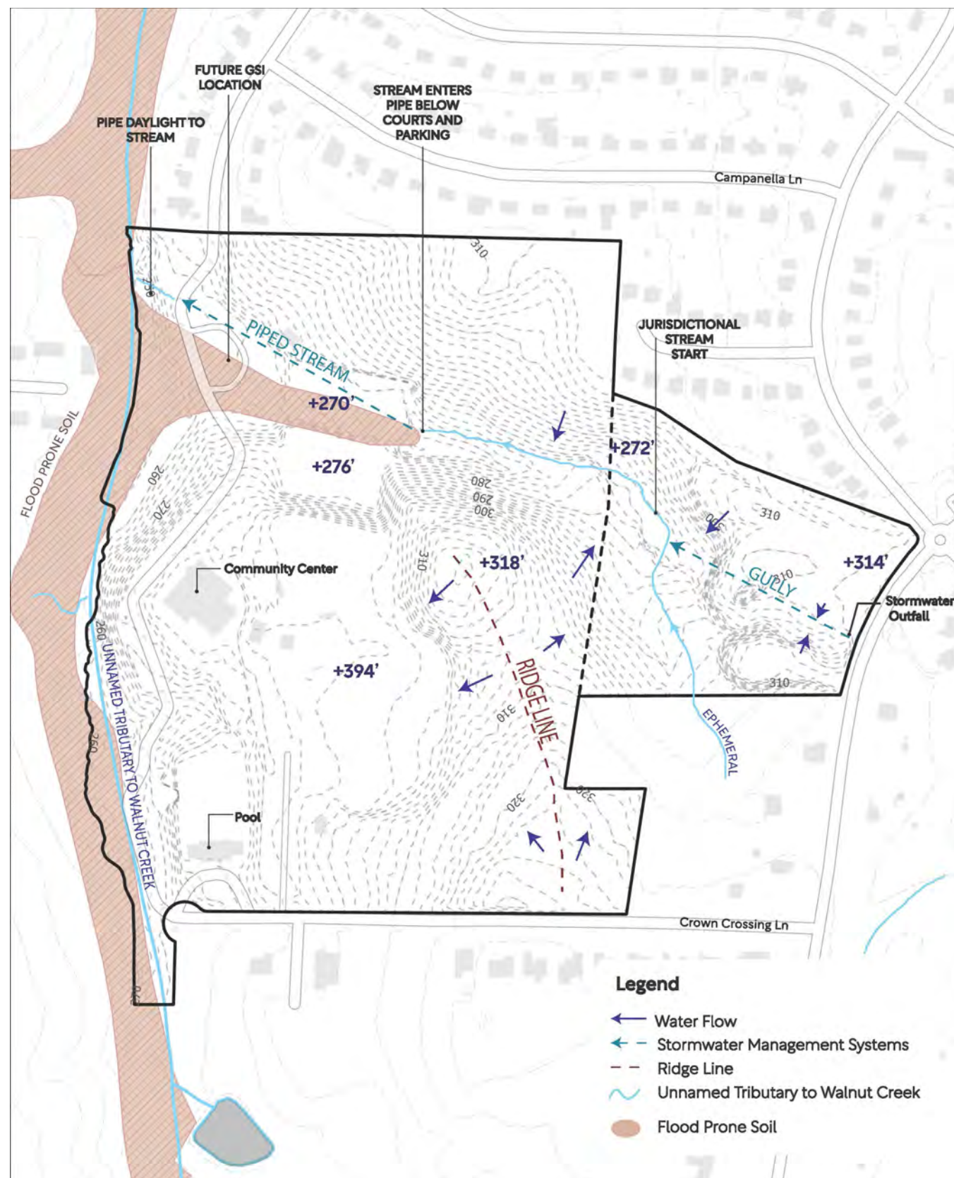
Site Hydrology Map; Runoff from Biltmore Hills Park joins the Walnut Creek to drain towards Rochester Heights
