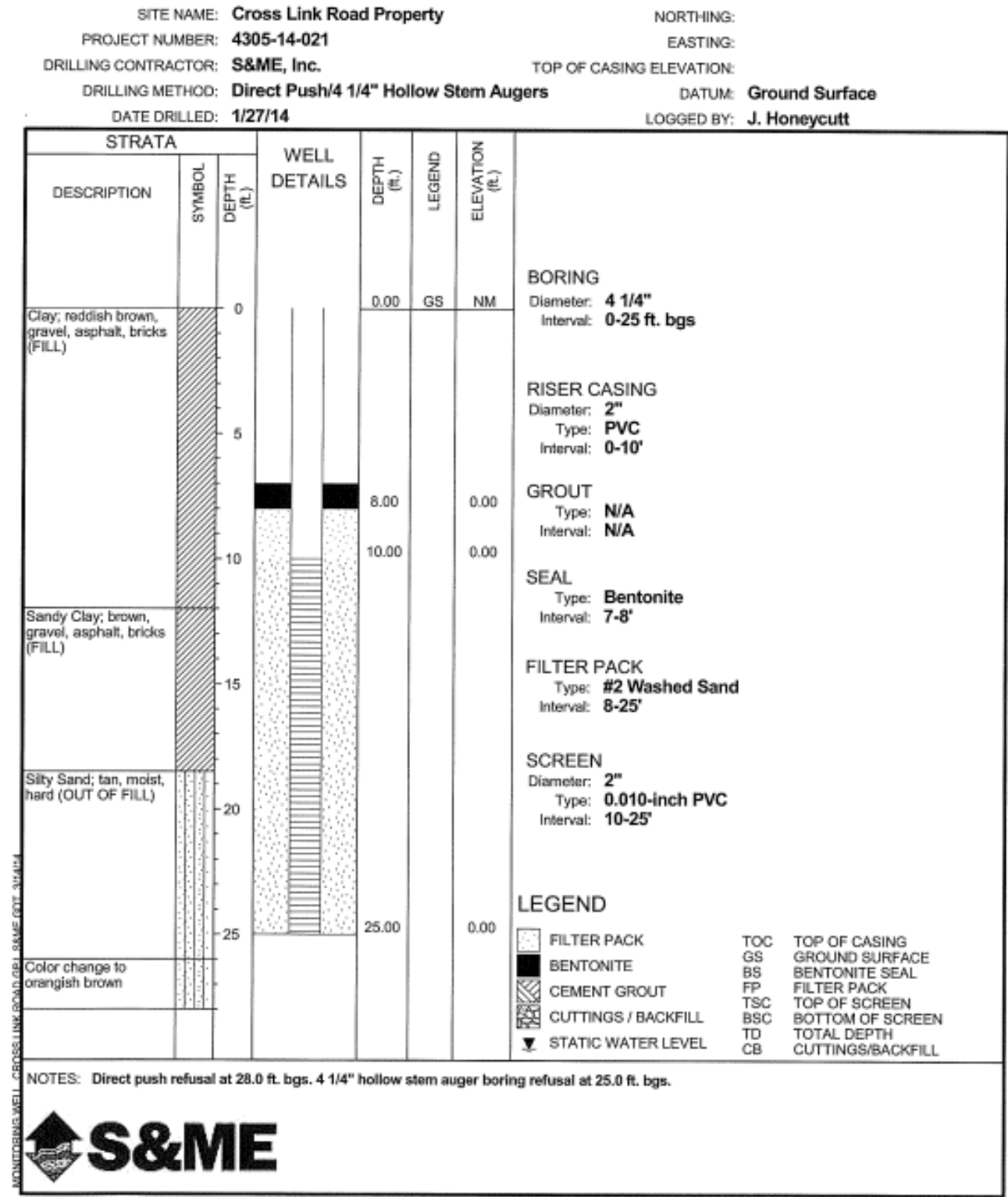
Boring Section at 1105 Cross Link Road; Approximately 18' of Fill then Transition to Native Soils
