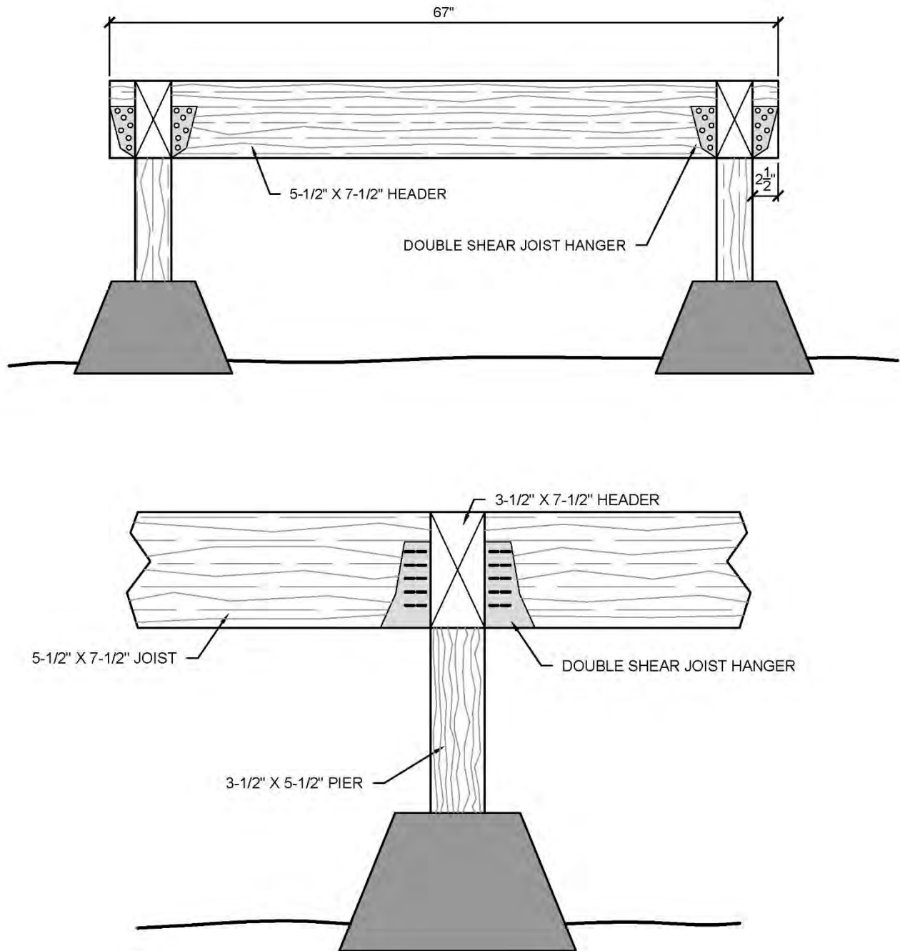
Figure 15.39 - Joist Attachment on Side of Header
