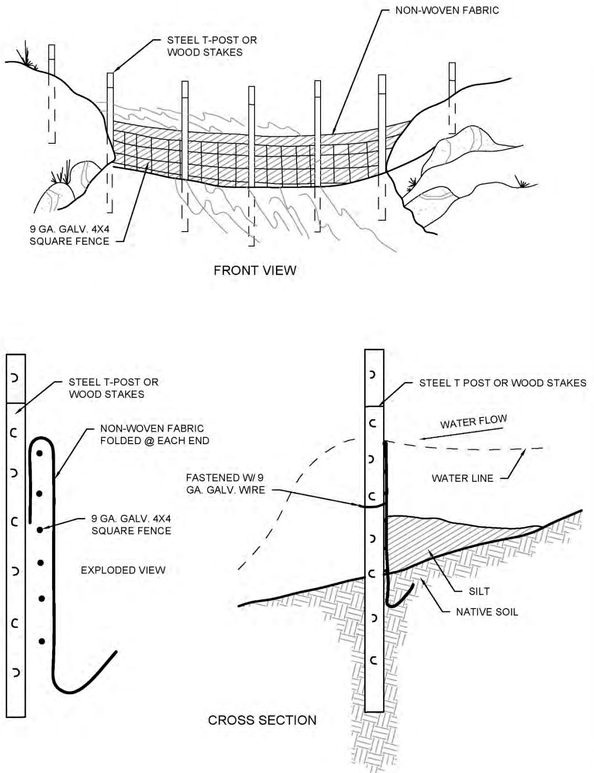
Figure 27.1 - Silt Fence
