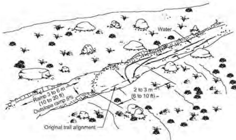
Figure 2: Diagram of a rolling grade dip
