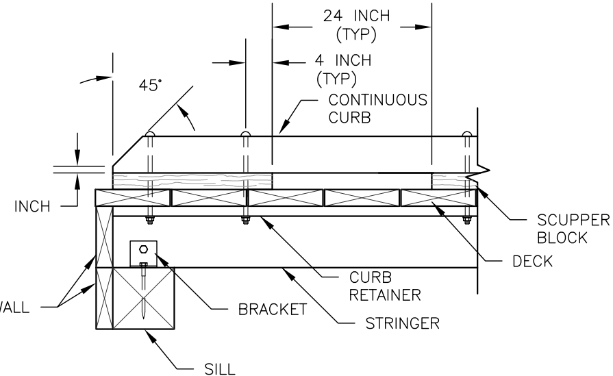
CURB DETAILS
