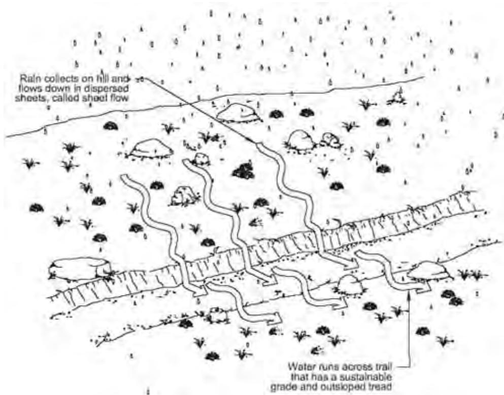
Figure 3: Diagram of sheet flow across a trail with gentle outsloping
