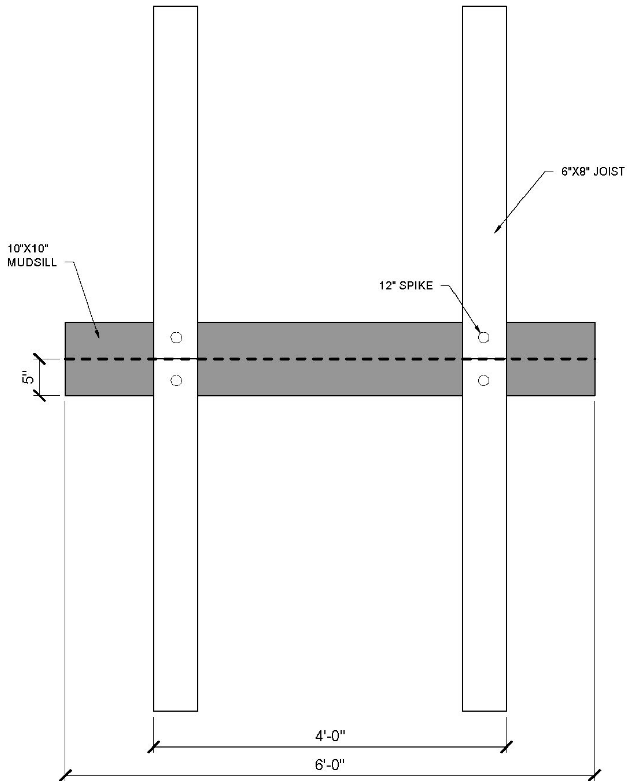
Figure 15.15 - Installing Multiple Puncheon Sections
