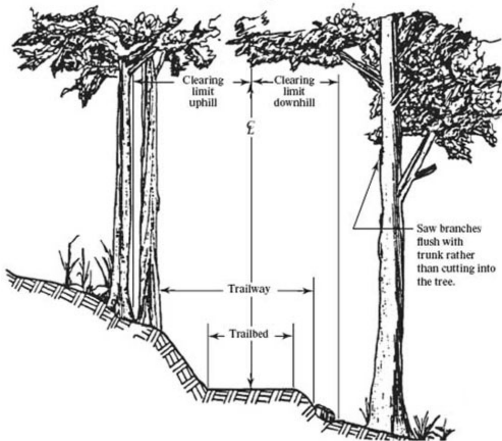
Figure 1: Diagram of trail clearing cross section
