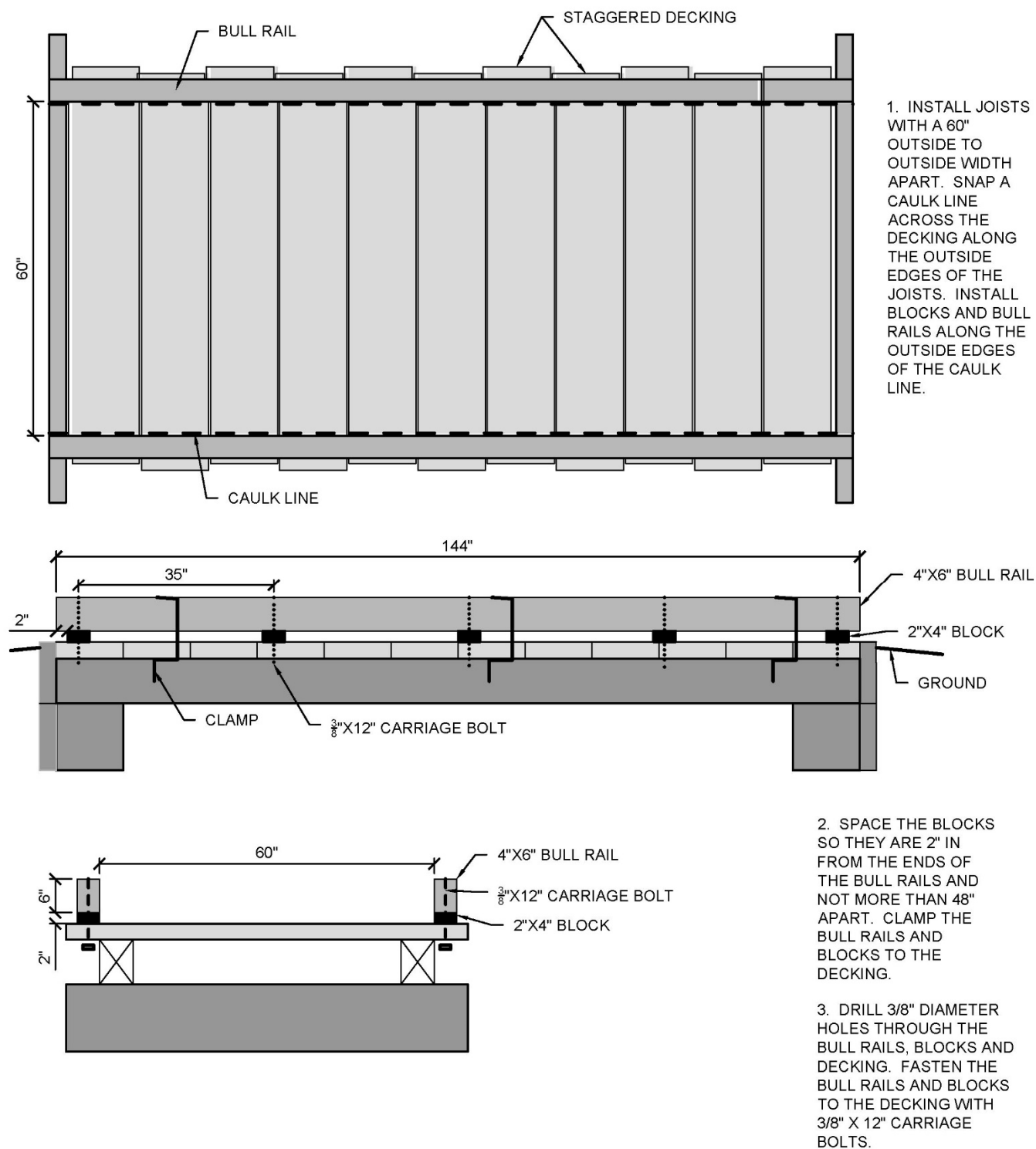
Figure 15.14 - Installing Bull Rails
