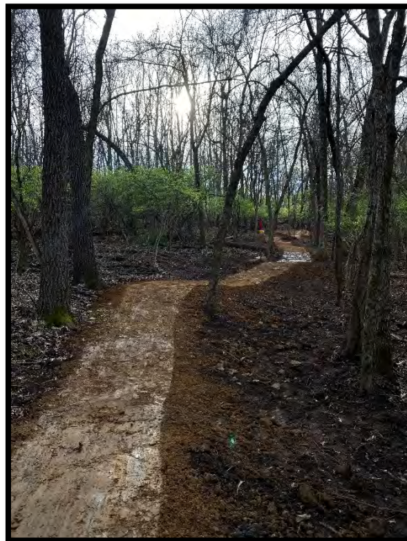
Figure 4: Conceptual experience representing Turnpike Tread construction seen in areas with flatter natural cross slopes.
