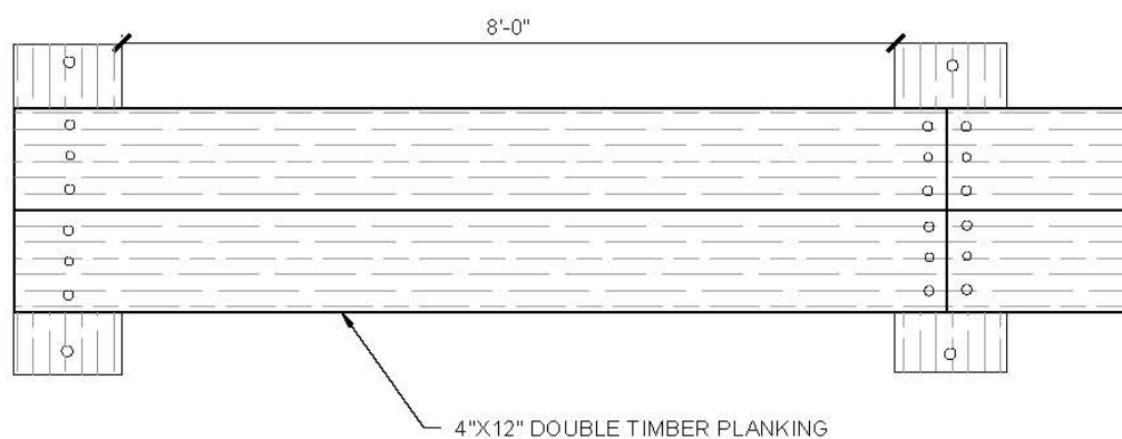
Figure 15.1 - Timber Planking
