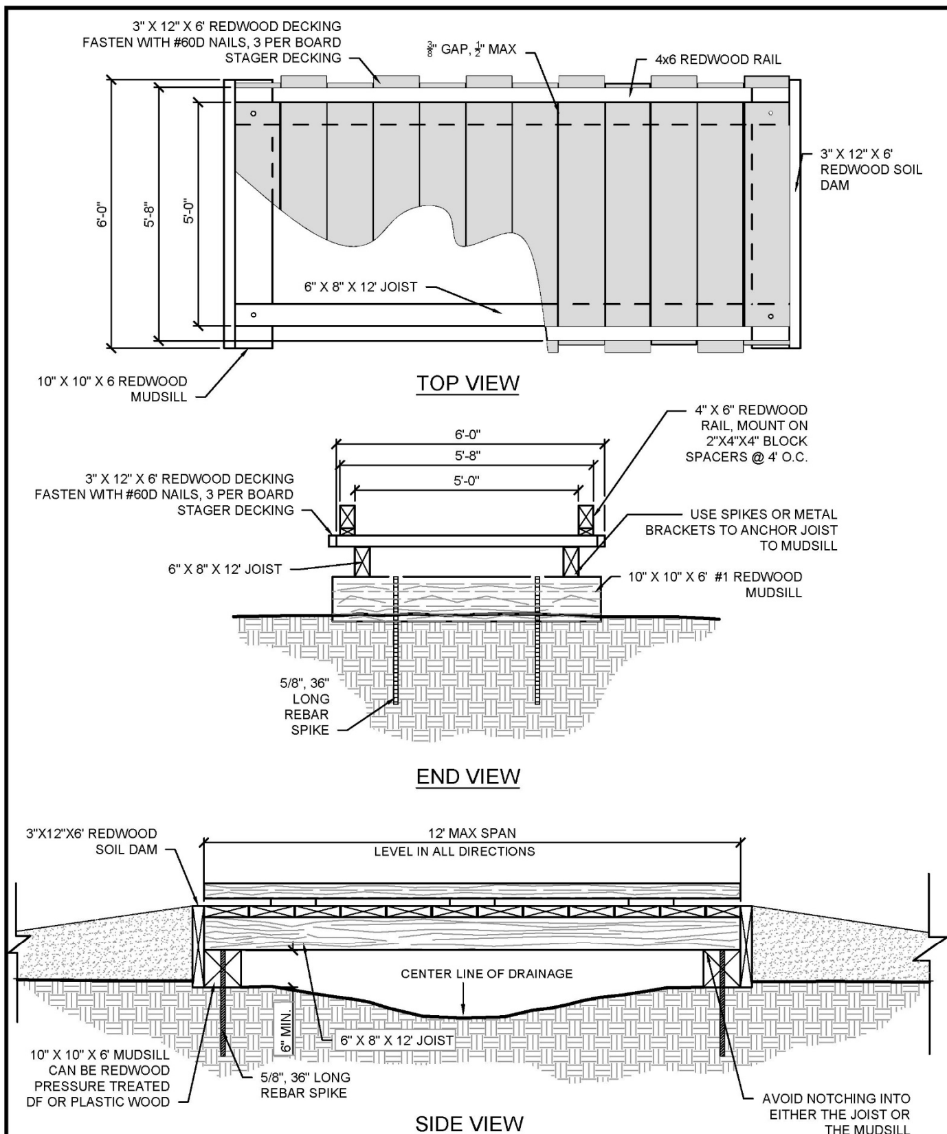
Figure 15.3 - Puncheon Structures
