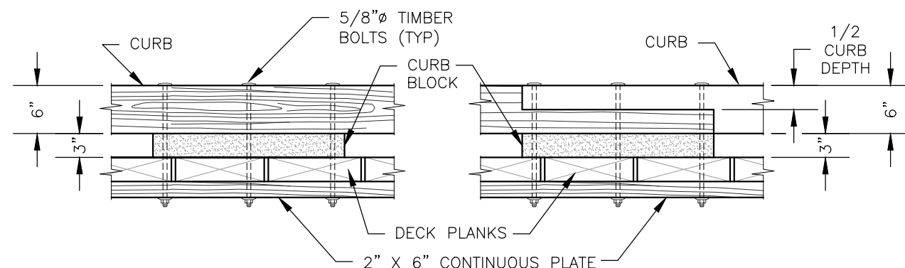
ELEVATION—TYPICAL CONNECTION
