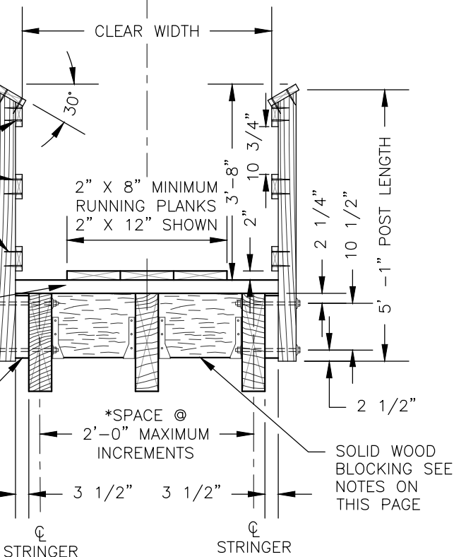
TYPICAL DECK SECTION W/RAILING SYSTEM
