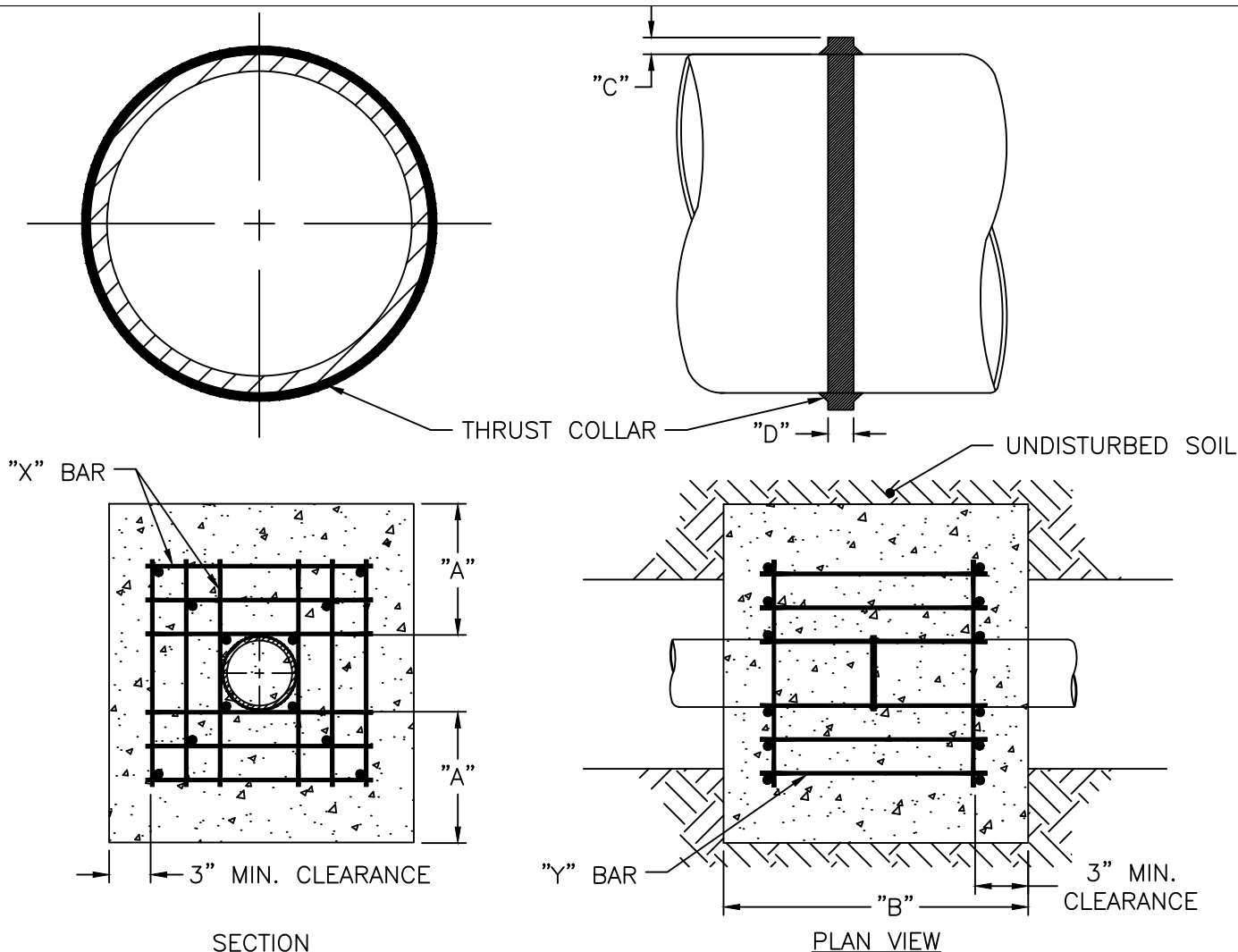
THRUST COLLAR AND THRUST SCHEDULE
