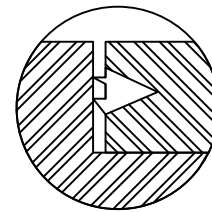
GASKET IN VERTICAL FACE OF COVER
