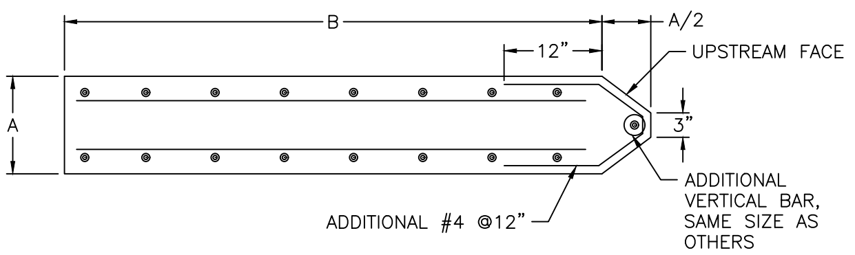
PLAN - CONCRETE SUPPORT NOSING (WHEN EXPOSED TO STREAM FLOW)
